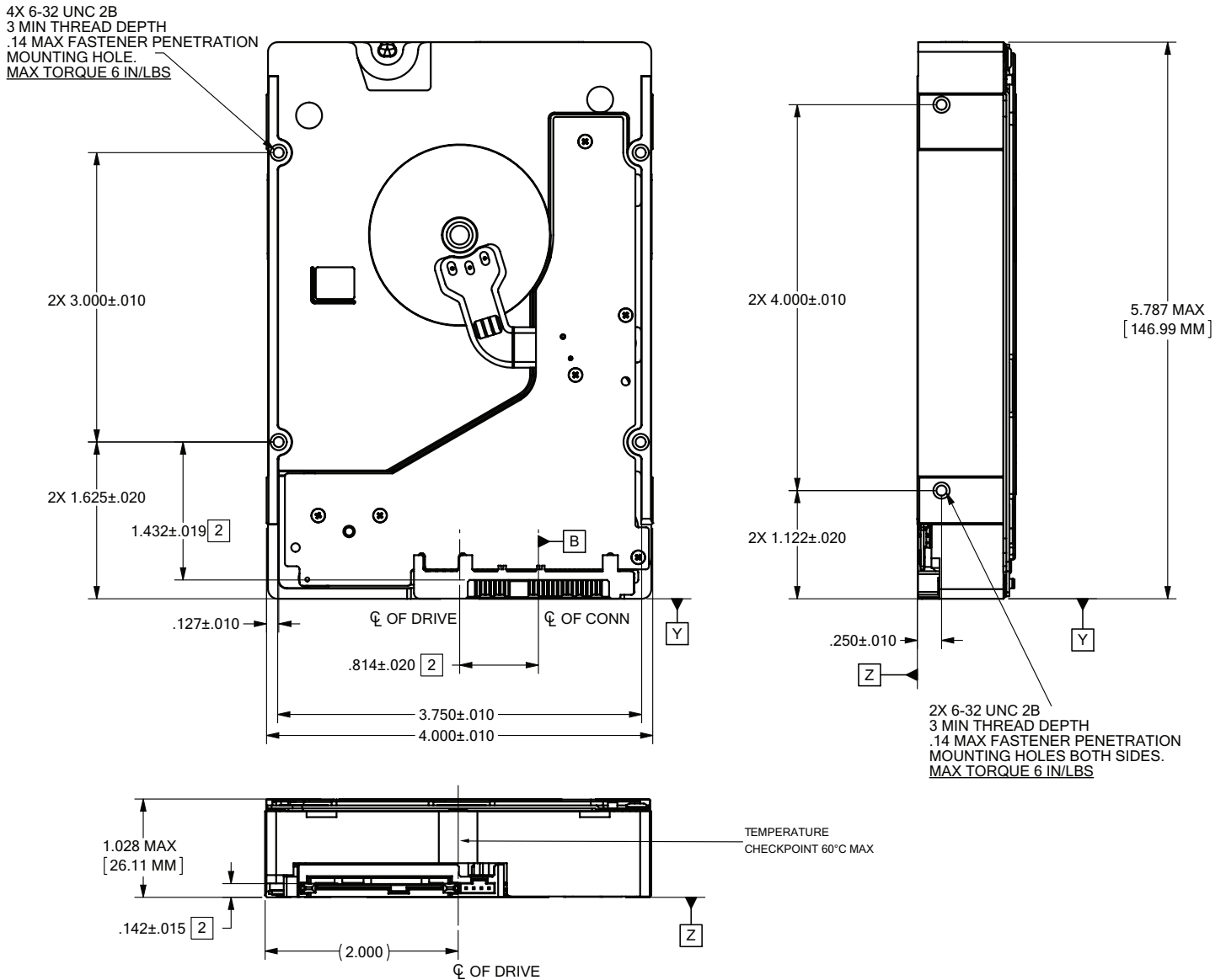
Figure 4. Mounting configuration dimensions (8TB and 6TB models)
