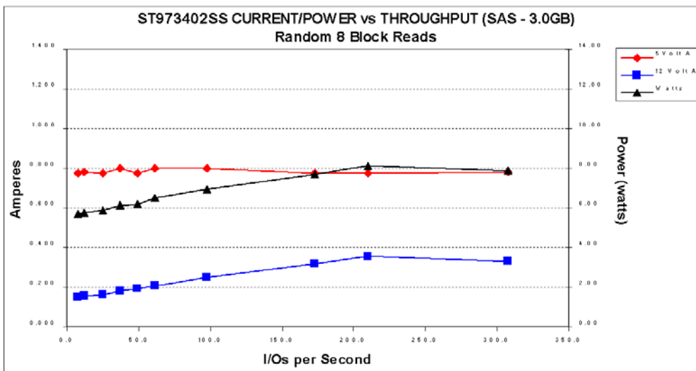
Figure 5. ST973402SS (3Gb) DC current and power vs. input/output operations per second
