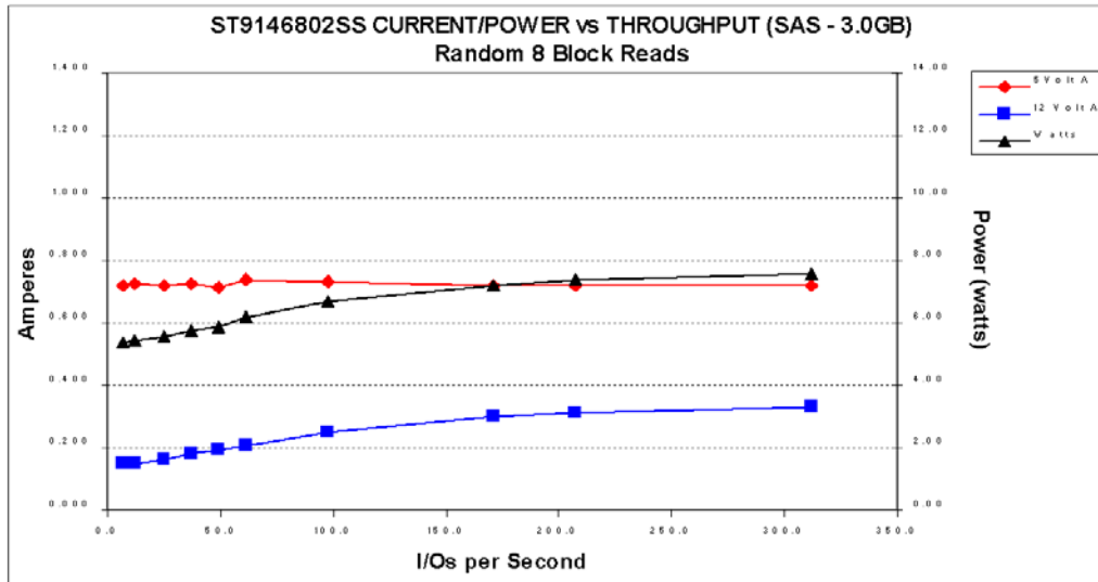
Figure 4. ST9146802SS (3Gb) DC current and power vs. input/output operations per second
