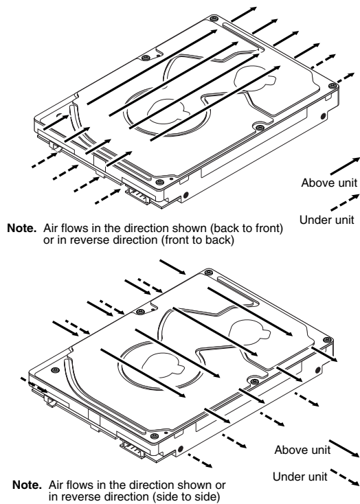
Figure 10. Air flow
