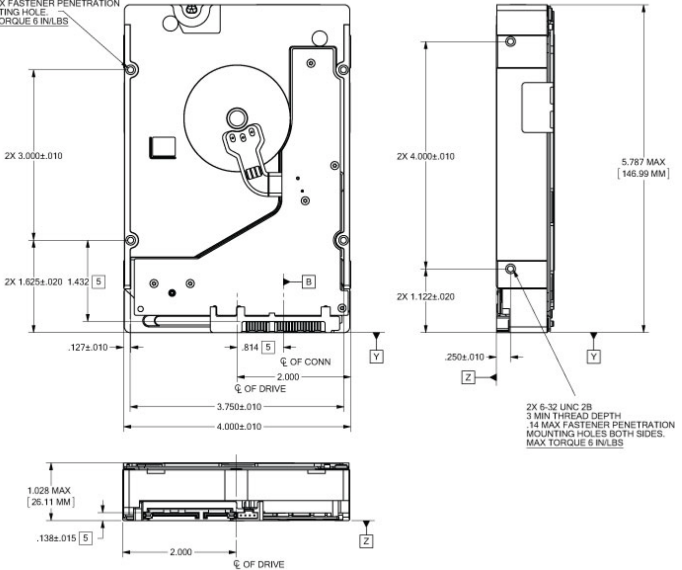
Figure 5. Mounting configuration dimensions for 10TB & 8TB models)
