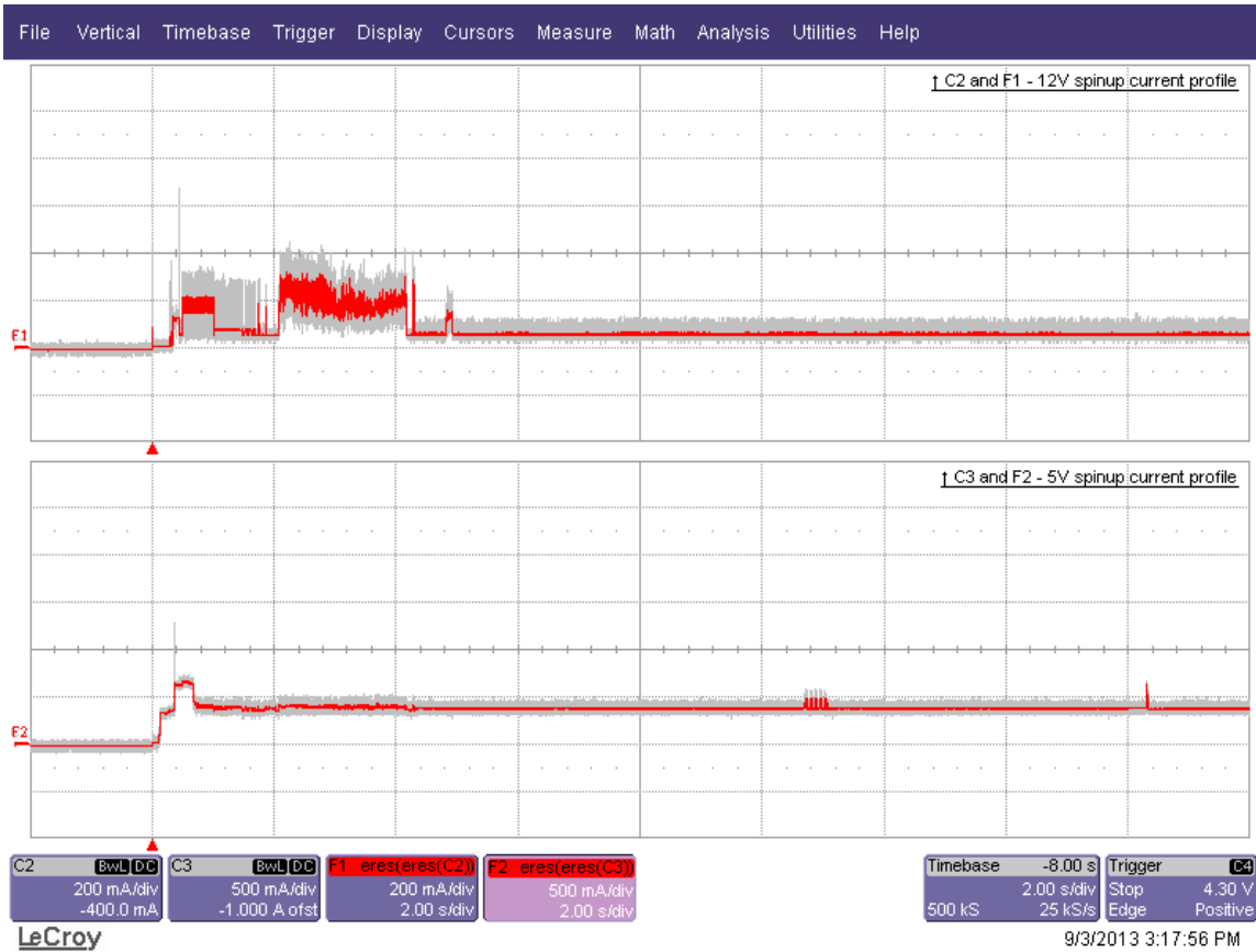
Figure 16. Current profiles for 400GB standard and 200GB high endurance models
